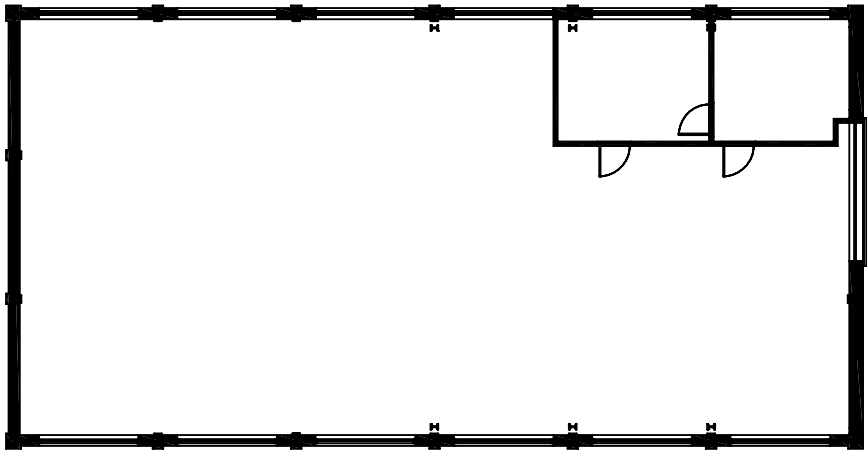
Plan approx 1:200
